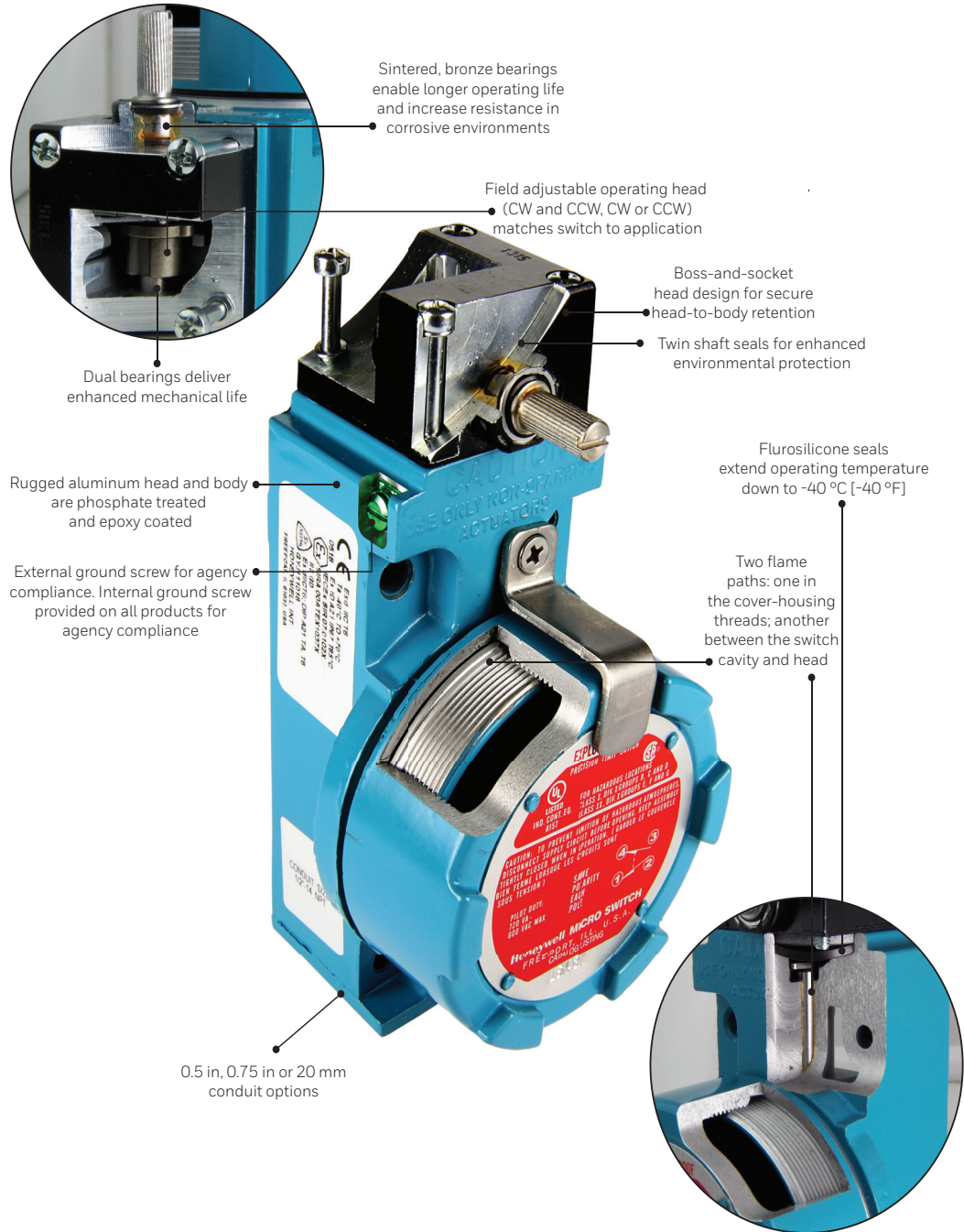
Figure 3. Honeywell's MICRO SWITCH BX/BX2 Series of hazardous location limit switches can be used in many hazardous or explosive environments around the globe. They offer a variety of options for actuators, housing materials, contacts, and sealings, as well as meet global certifications.
