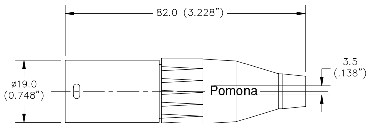
Model 5110 3-Pin XLR (M), silver contacts, nickel shell
