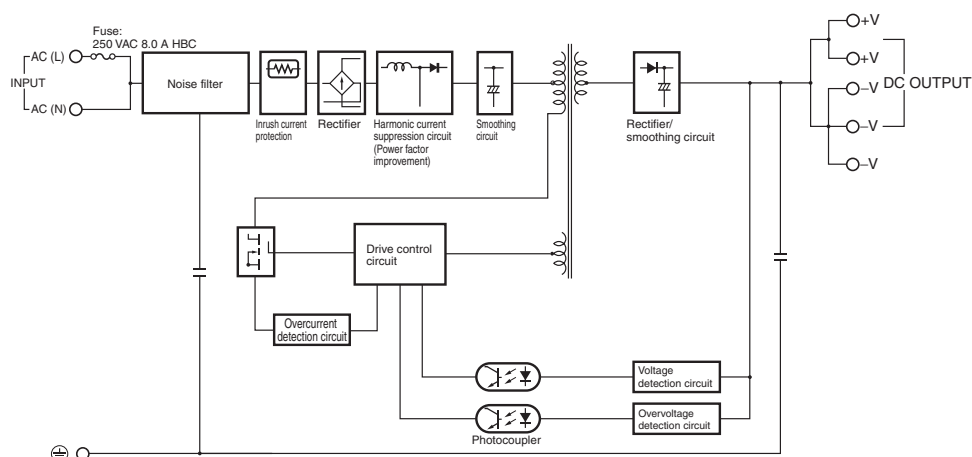
S8VK-C24024 (240W)
