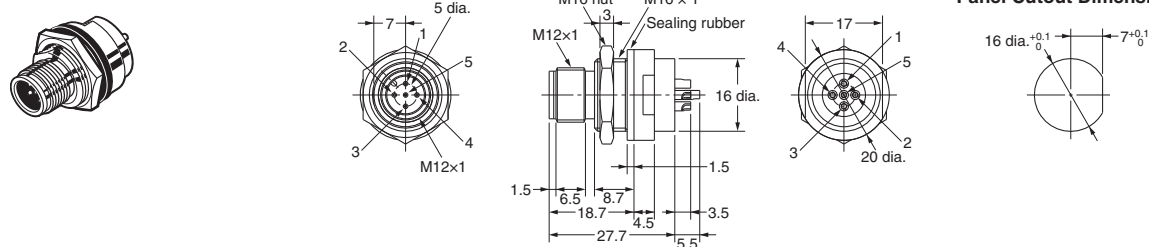
Panel Cutout Dimensions
