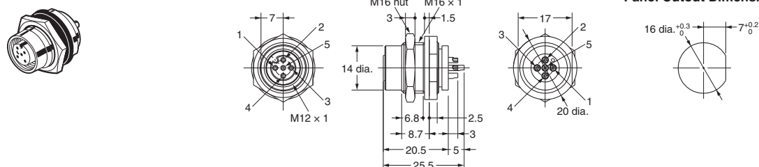
Panel Cutout Dimensions
