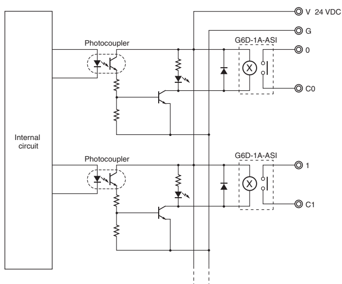
GT1-ROS16
