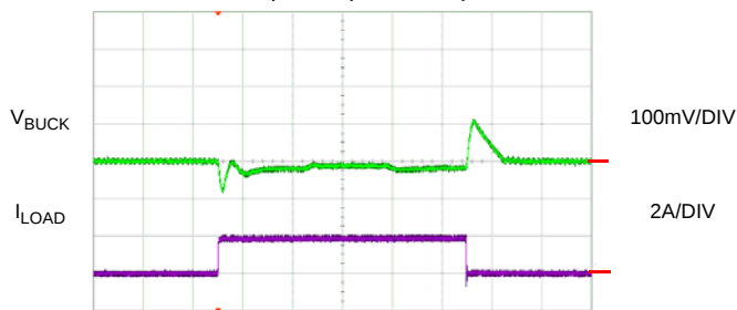
Load Transient Response (Additional Output Capacitance)
