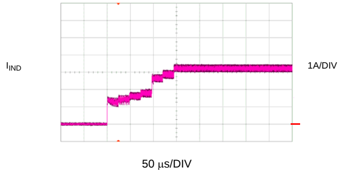
88MG830 Soft Start Current Limit (See Note)
