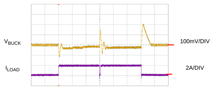
Double-Pulsed Load Response
