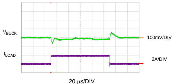
Load Transient Response (2 x Additional Output Capacitance)
