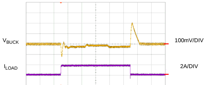
Load Transient Response
