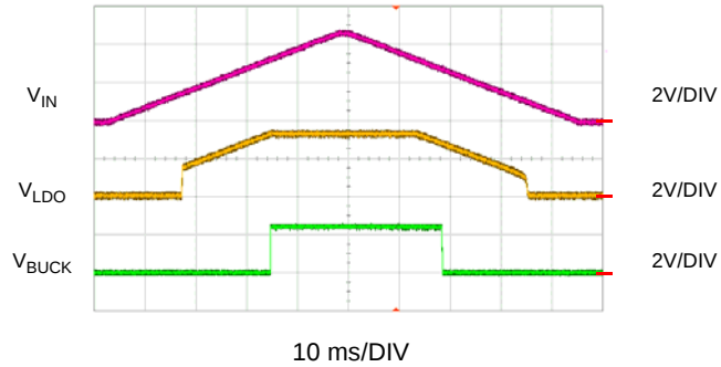
UVLO Thresholds
