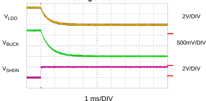
Turn Off Using the Shutdown Pin
