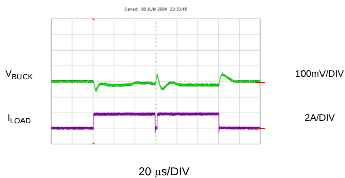
Double-Pulsed Load Response
