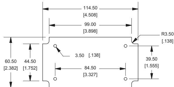
END VIEW OF ENCLOSURE
