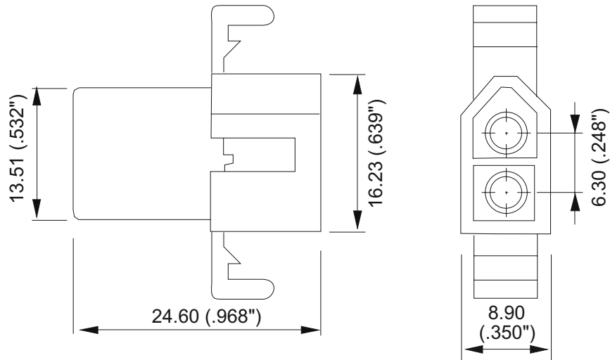
Plug ( 37-302-0 )
