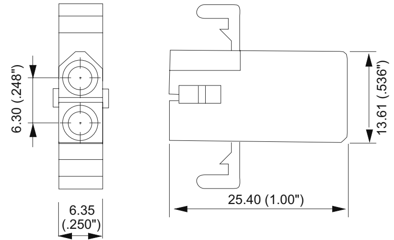
Receptacle ( 37-402-0 )
