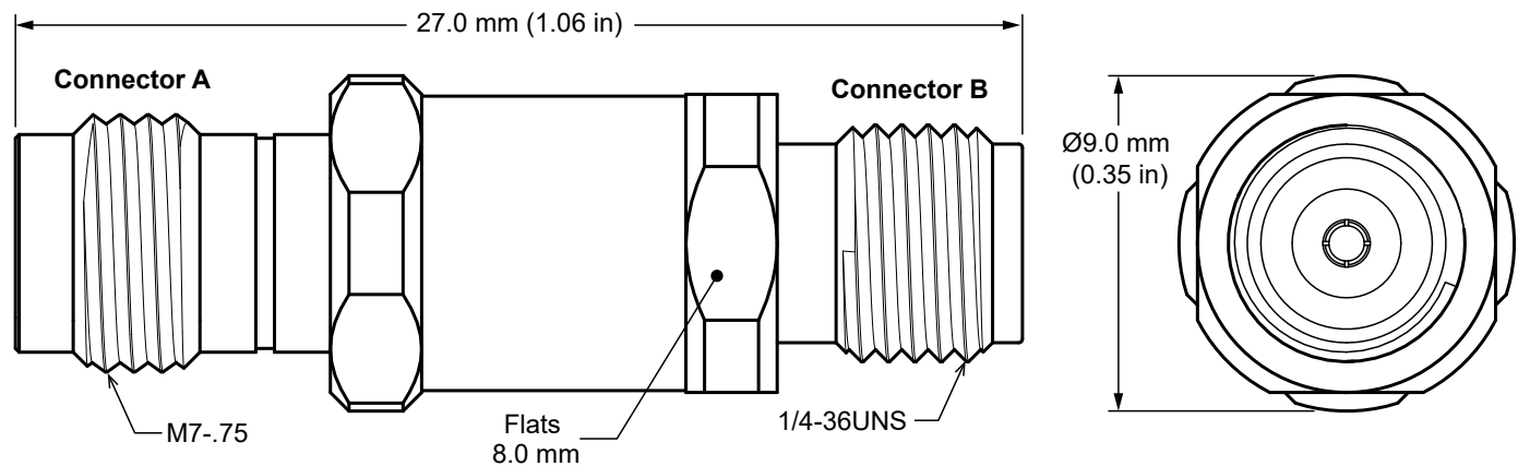
Figure 1: Product Dimensions for the ADP-2.4F-2.92F Adapter
