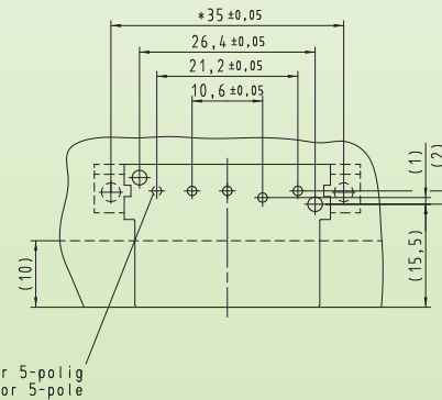
4/5-pole
