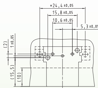
3-pole
