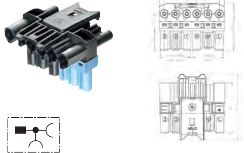
T distributor
