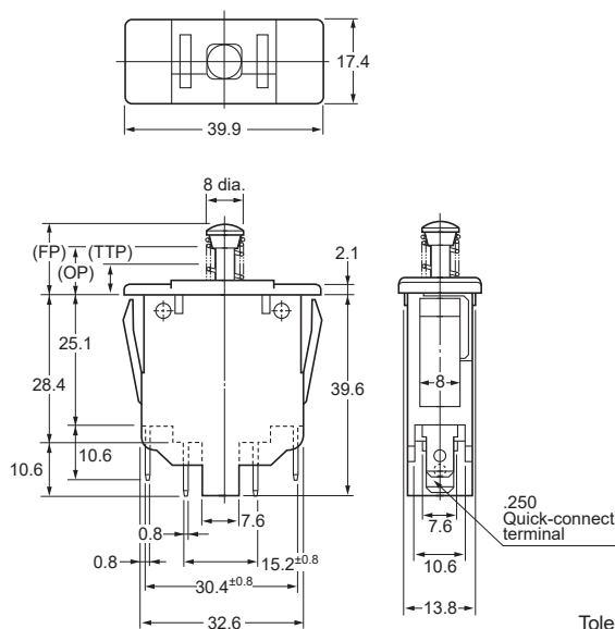
2 Form A type without button guard
