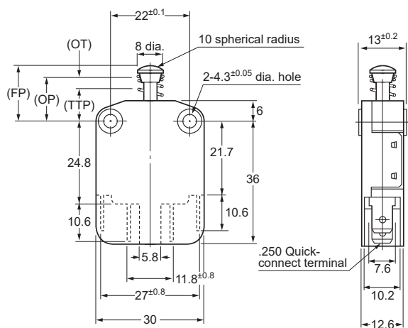
External dimensions
