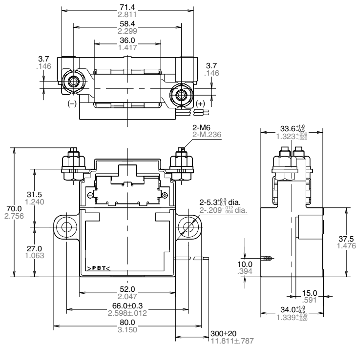
External dimensions
