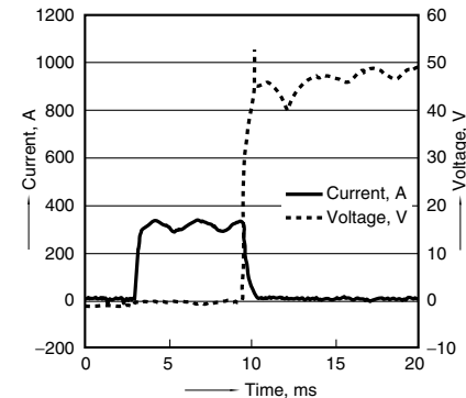
(1) Cut off current/voltage: 300A/42V DC (resistive load)
