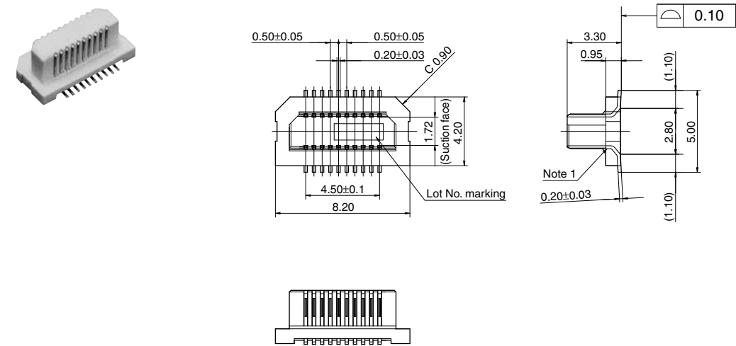
External dimensions
