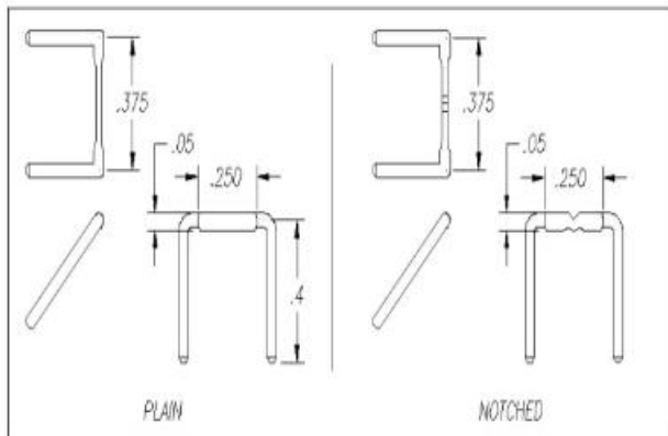
Ni-Chrome Wirestripping Elements (Flat, Single Notched) Model 10529
