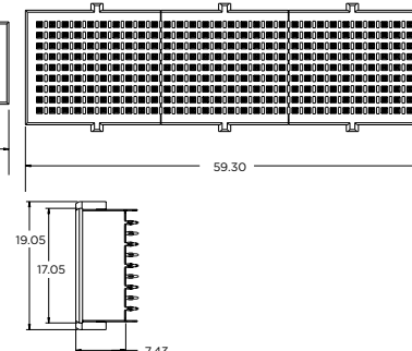
Nine-Row Connectors
